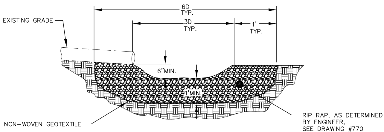
PROFILE
