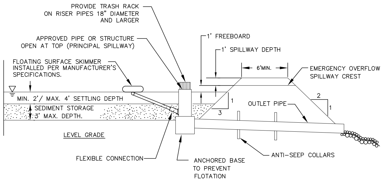
PROFILE
