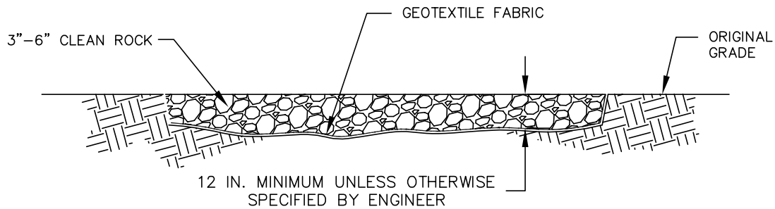
SECTION B-B
