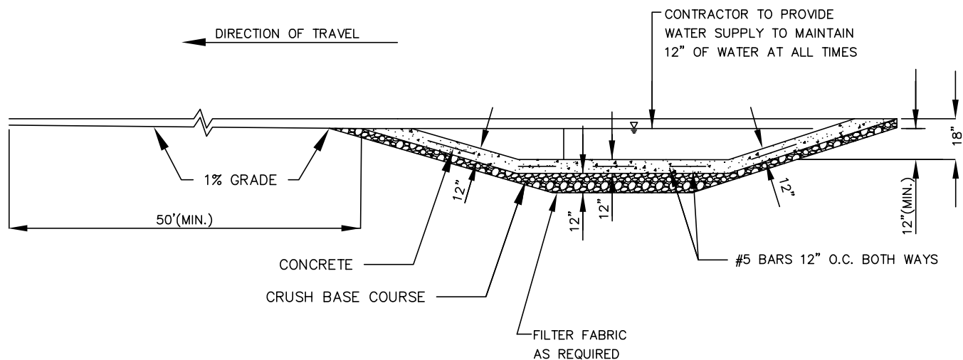
PROFILE
